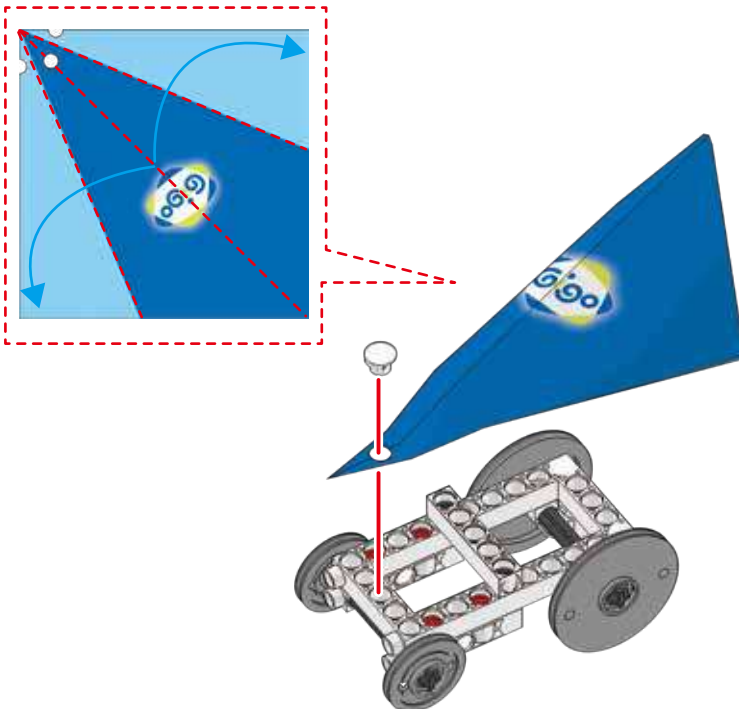
4-2 Windsurfing Sail Car
